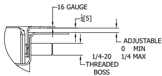
DETAIL F
