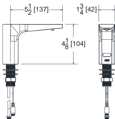
DISPENSER SPOUT
