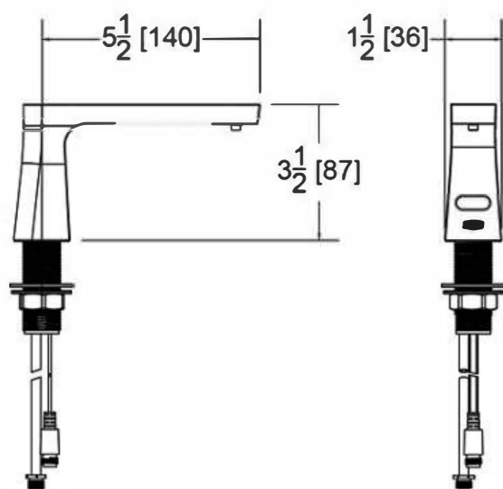
DISPENSER SPOUT
