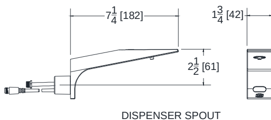
DISPENSER SPOUT
