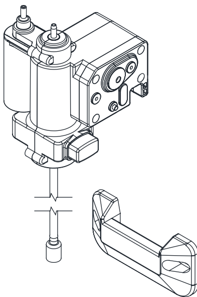
Control Box Assembly & Mounting Bracket
