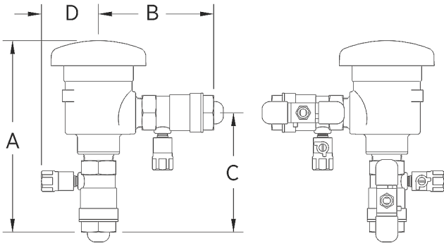
Dimensions & Weights (do not include pkg.)
