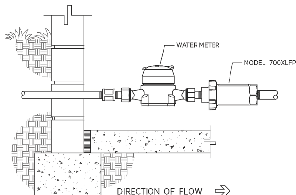
INDOOR INSTALLATION
