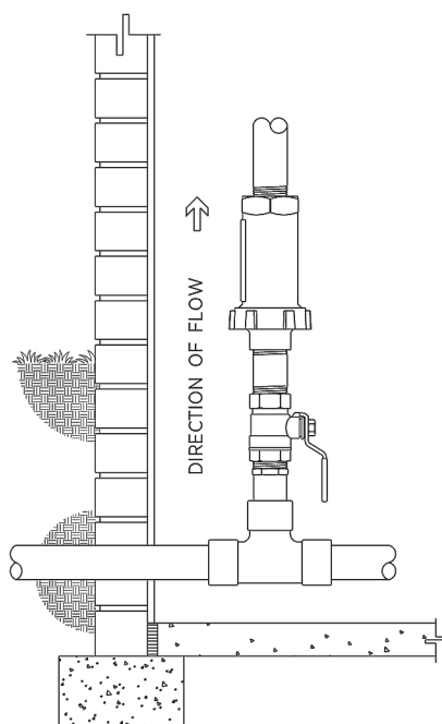
VERTICAL INSTALLATION
