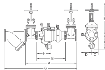
MODEL 375A with OSY & FSC option
