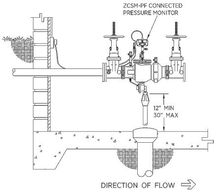
INDOOR INSTALLATION
