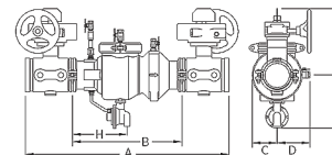
MODEL 375A with BG option
