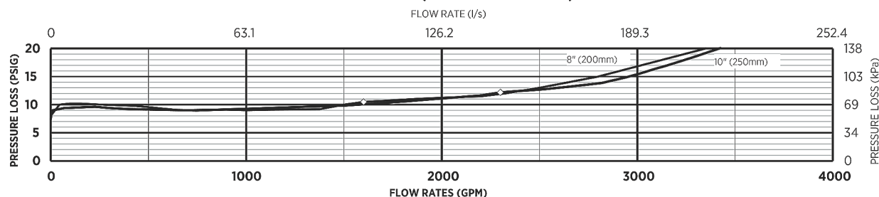
MODEL 375A 8" & 10" (STANDARD AND METRIC)
