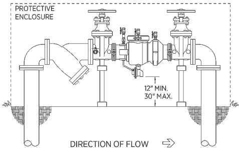
OUTDOOR INSTALLATION
