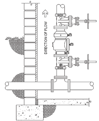
VERTICAL INSTALLATION (3500SYG)
