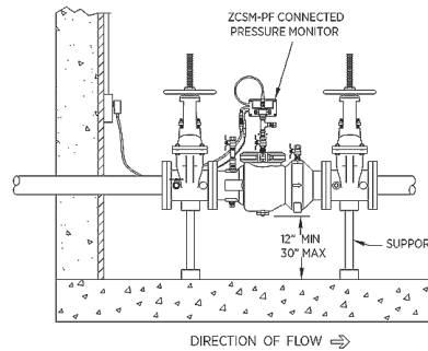
INDOOR INSTALLATION (3500SY with ZCSM-PF Connected Pressure Monitor)
