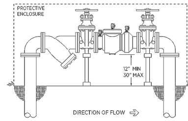
OUTDOOR INSTALLATION
