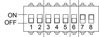
All switches shown in default mode.
